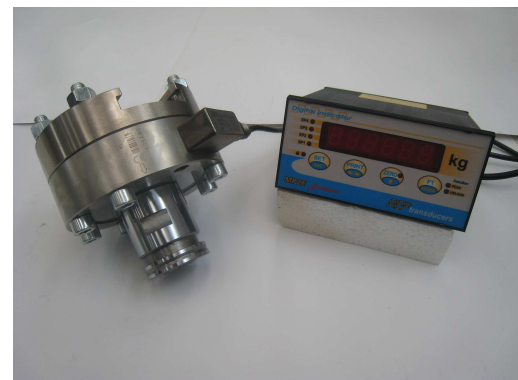
Load Cell
