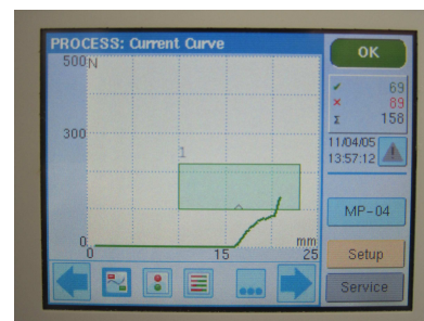
Thrust-Stroke Diagram
