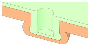
Clinching
